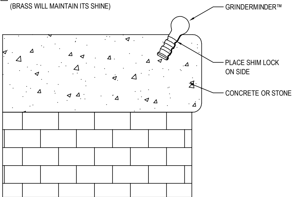
INSTALLATION DETAIL
